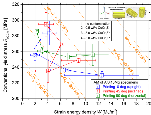
Fig. 5. Quality index analysis of the investigated cross-contamination levels and printing orientation.
